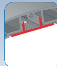
Assembly: Hidden aluminum connector with screw
