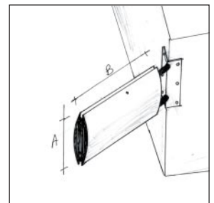
12. Installation on the corner of a building.
